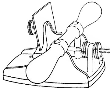
FIG. 79. VENEER SCRAPER.
